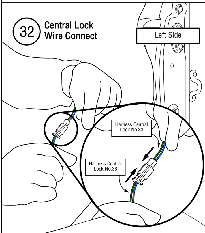
The process of connecting the Central Lock (BL,DG) wiring of the Harness Central Lock No.33 with the Central Lock (BL,DG) wiring of the Harness Central Lock No.38.
