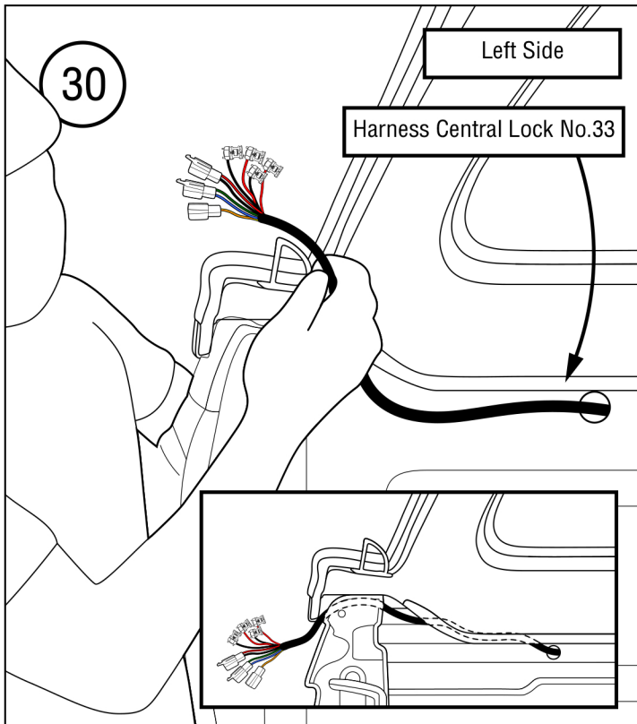
Running the Harness Central Lock No.33 along the vehicle tube through the rear light.
