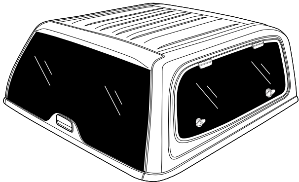
Backdoor
